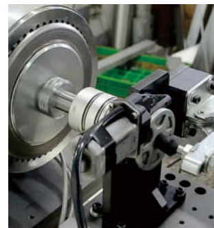
Multi-Torsion Testing
