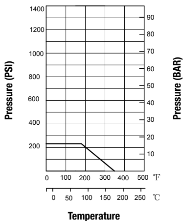
Pressure-Temp. Rating
